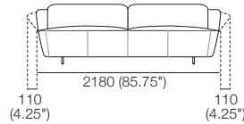
2.5 Seater Front View Backrest Down
