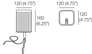
PocketAccessory SMART Speaker Bracket Pair Sonos Play 1 Side View / Top View
